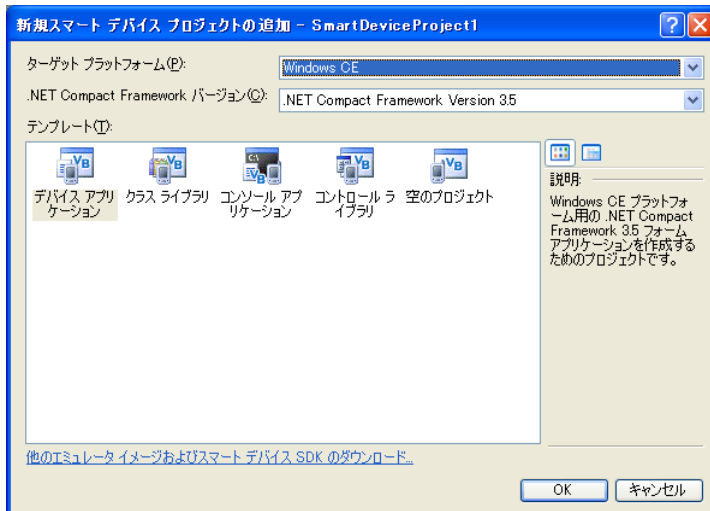
Visual Studio 2008
